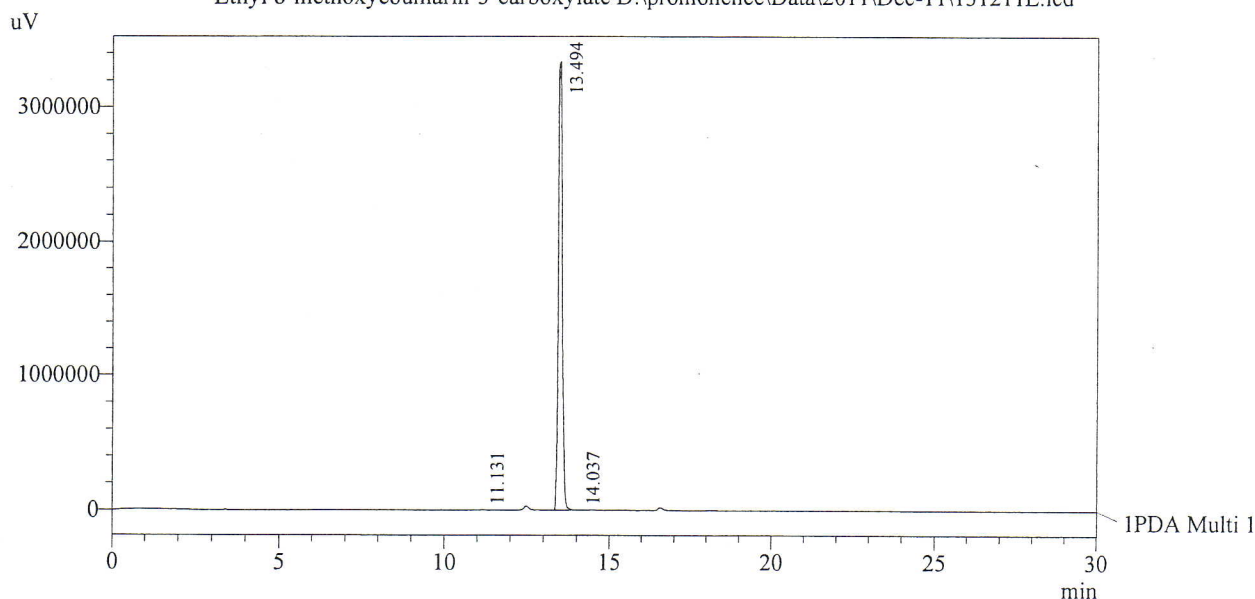
Chromatogram Ethyl 8-methoxycoumarin-3-carboxylate D:\promonence\Data\2011\Dec-11\131211E.lcd
